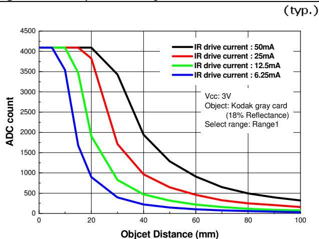
Fig.5 PS output vs. Object distance
