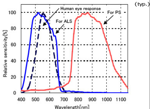
Fig.4 Spectral response
