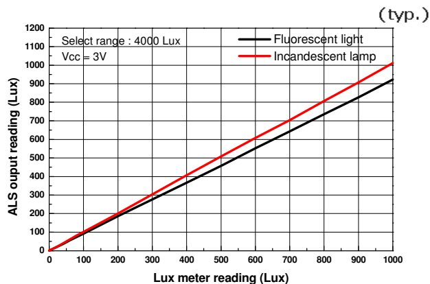
Fig.3 Sensitivity to different light source
