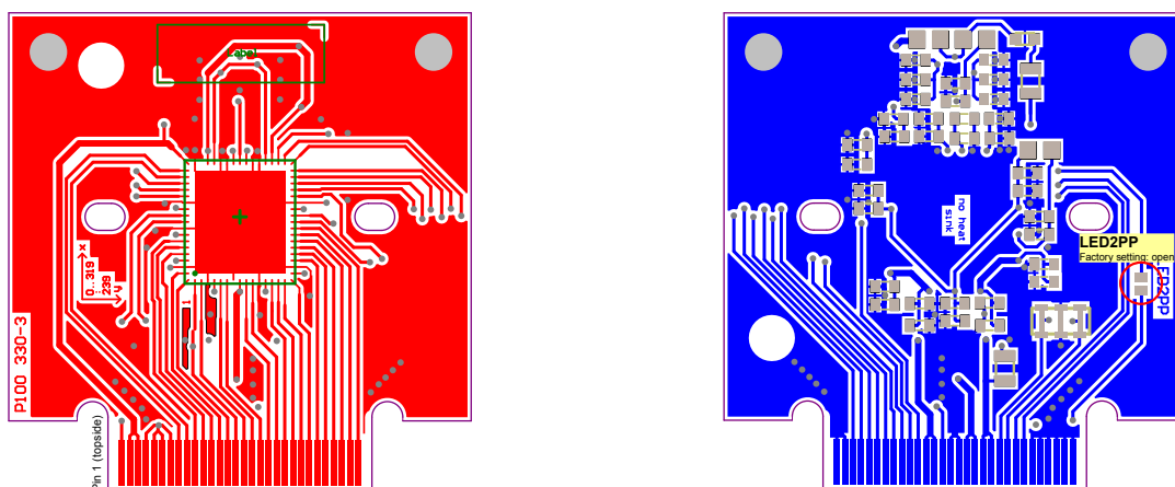
Figure 5: Layout top and bottom
