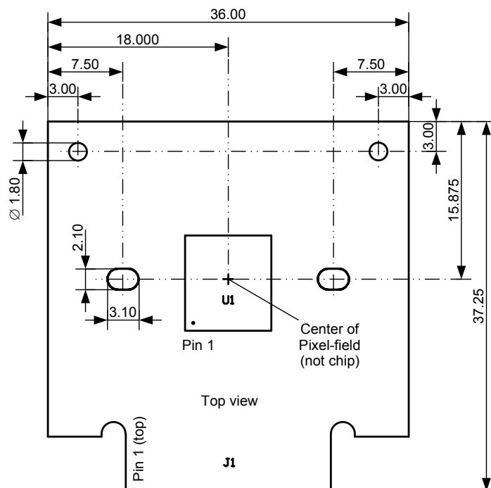
Figure 7: Dimensions in mm (PCB material is glass epoxy FR-4, thickness 1.6mm)
