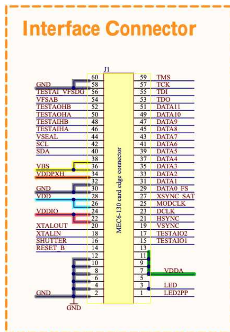
Figure 3: Schematic diagram - Card edge Connector
