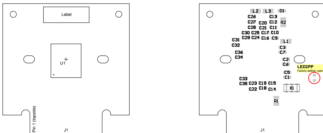
Figure 6: Assembly top and bottom
