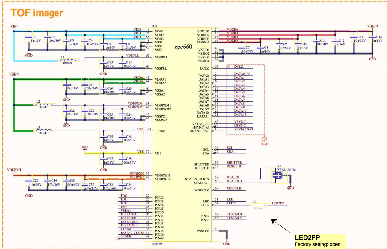
Figure 2: Schematic diagram - TOF imager
