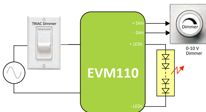
APPLICATION DIAGRAM
