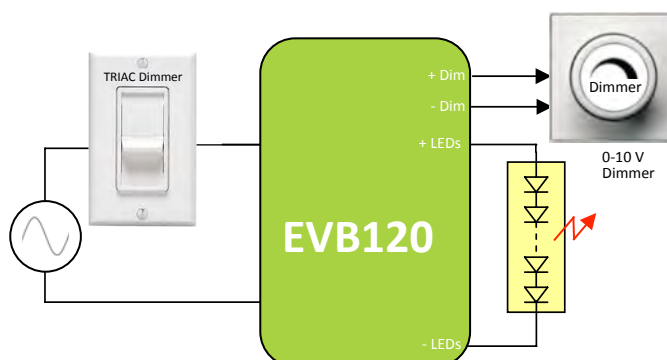
APPLICATION DIAGRAM
