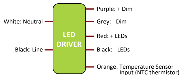
WIRING DIAGRAM
