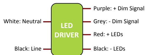
WIRING DIAGRAM
