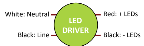
WIRING DIAGRAM
