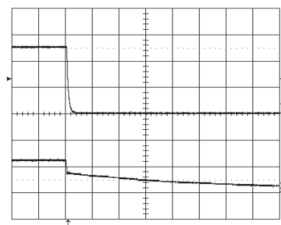
Turn-off at I_O = 16\text{ A} resistive load at T_{ref} = +25\text{ }^{\circ}\text{C} , V_{in} = 12\text{ V} . Turn-off enabled by disconnecting V_{in} . Top trace: output voltage (2 V/div.). Bottom trace: input voltage (10 V/div.). Time scale: 2 ms/div.
