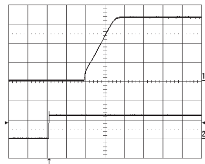
Start-up at I_O = 16\text{ A} resistive load at T_{ref} = +25\text{ }^{\circ}\text{C} , V_{in} = 12\text{ V} . Start enabled by connecting V_{in} . Top trace: output voltage (1 V/div.). Bottom trace: input voltage (10 V/div.). Time scale: 2 ms/div.
