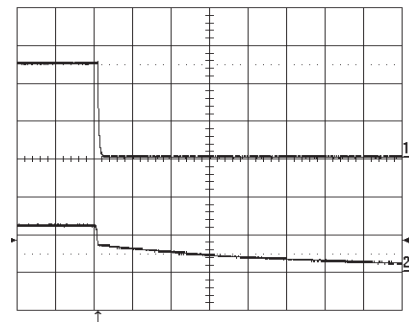
Turn-off at I_O = 16\text{ A} resistive load at T_{ref} = +25\text{ }^{\circ}\text{C} , V_{in} = 12\text{ V} . Turn-off enabled by disconnecting V_{in} . Top trace: output voltage (1 V/div.). Bottom trace: input voltage (10 V/div.). Time scale: 2 ms/div.
