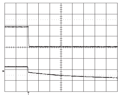
Turn-off at I_O = 16\text{ A} resistive load at T_{ref} = +25\text{ }^{\circ}\text{C} , V_{in} = 12\text{ V} . Turn-off enabled by disconnecting V_{in} . Top trace: output voltage (1 V/div.). Bottom trace: input voltage (10 V/div.). Time scale: 2 ms/div.
