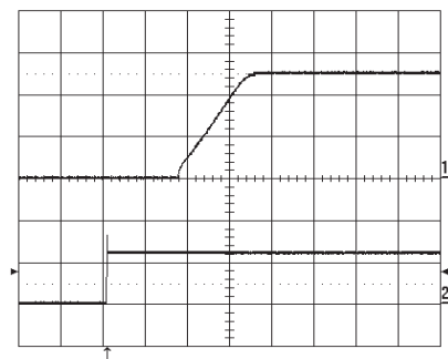
Start-up at I_O = 16\text{ A} resistive load at T_{ref} = +25\text{ }^{\circ}\text{C} , V_{in} = 12\text{ V} . Start enabled by connecting V_{in} . Top trace: output voltage (2 V/div.). Bottom trace: input voltage (10 V/div.). Time scale: 2 ms/div.
