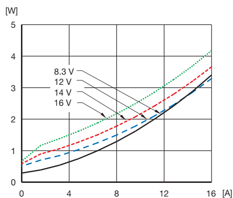
Dissipated power vs. load current and input voltage at T_{ref} = +25^\circ\text{C}
