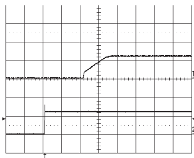
Start-up at I_O = 16\text{ A} resistive load at T_{ref} = +25^\circ\text{C} , V_{in} = 12\text{ V} . Start enabled by connecting V_{in} . Top trace: output voltage (1 V/div.). Bottom trace: input voltage (10 V/div.). Time scale: 2 ms/div.
