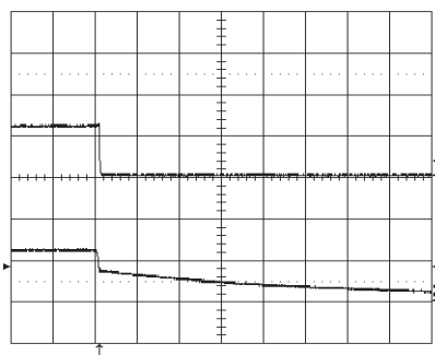
Turn-off at I_O = 16\text{ A} resistive load at T_{ref} = +25^\circ\text{C} , V_{in} = 12\text{ V} . Turn-off enabled by disconnecting V_{in} . Top trace: output voltage (1 V/div.). Bottom trace: input voltage (10 V/div.). Time scale: 2 ms/div.
