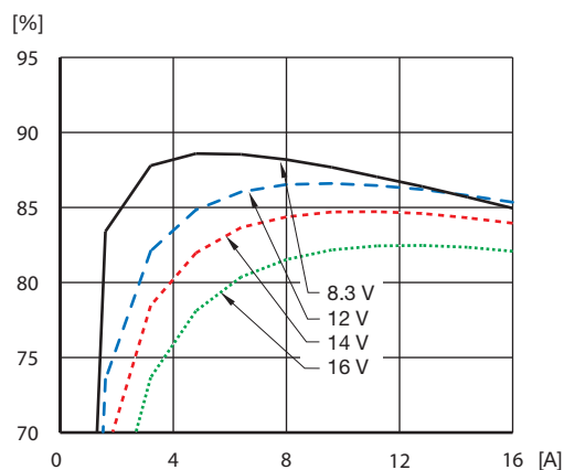
Efficiency vs. load current and input voltage at T_{ref} = +25^\circ\text{C}
