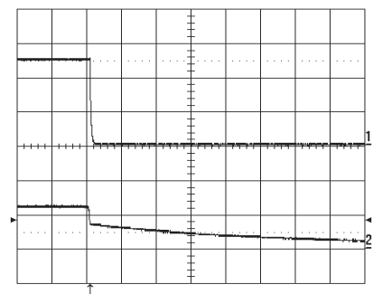
Turn-off at I_O = 10\text{ A} resistive load at T_{ref} = +25\text{ }^{\circ}\text{C} , V_{in} = 12\text{ V} . Turn-off enabled by disconnecting V_{in} . Top trace: output voltage (1 V/div.). Bottom trace: input voltage (10 V/div.). Time scale: 2 ms/div.
