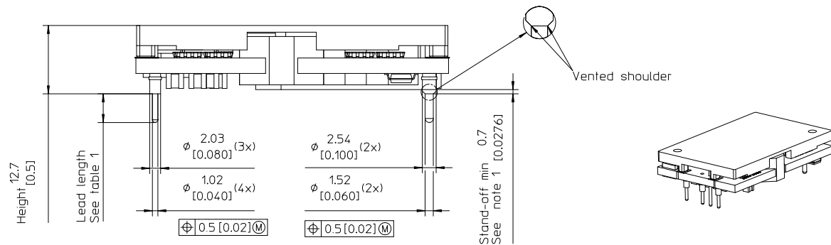
TOP VIEW
