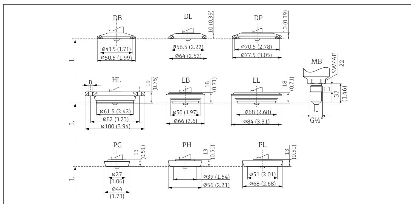
7 Process connection versions
