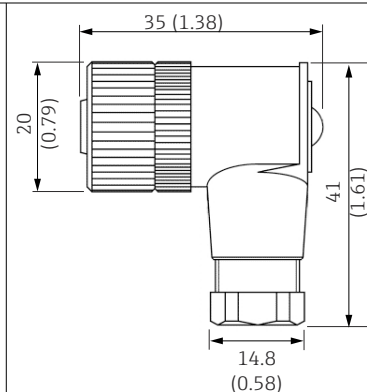
13 Dimensions in mm (in)
