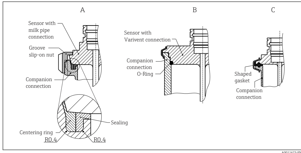
3 Detailed installation instructions for hygiene-compliant installation
