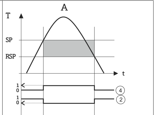
8 Switch point functions
