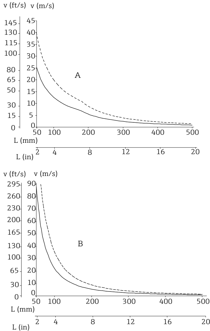
8 Maximum flow velocity with thermowell diameter 9 mm (0.35 in) (—) or 12 mm (0.47 in) (-----)
