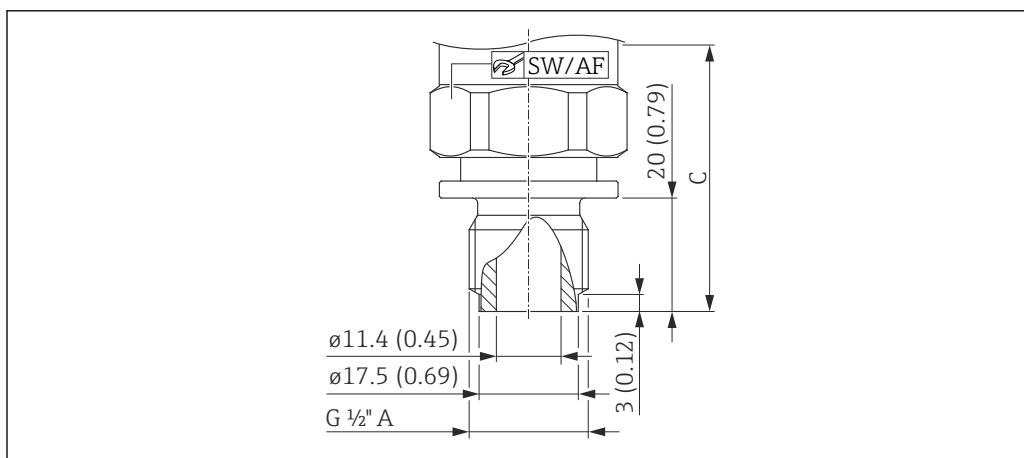
6 Thread ISO 228 G 1/2" A, bore 11.4 mm (0.45 in). Unit of measurement mm (in)
