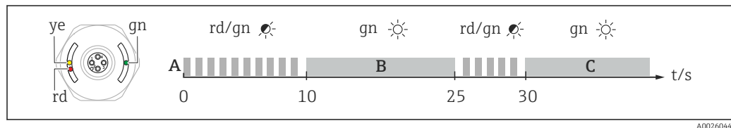
5 Time diagram for settings and default value
