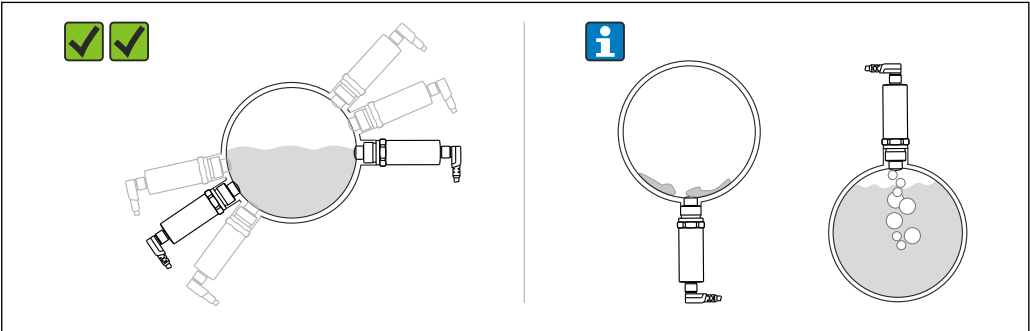
2 Installation in horizontal pipes
