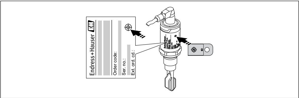
29 Position for test magnet on housing
