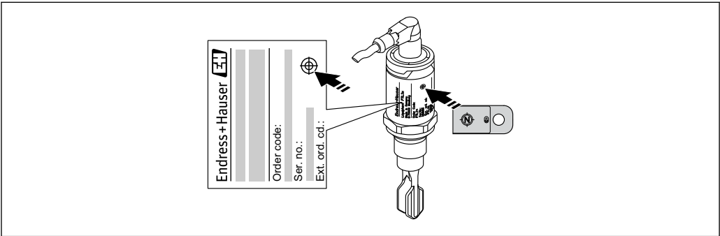
23 Position for test magnet on housing
