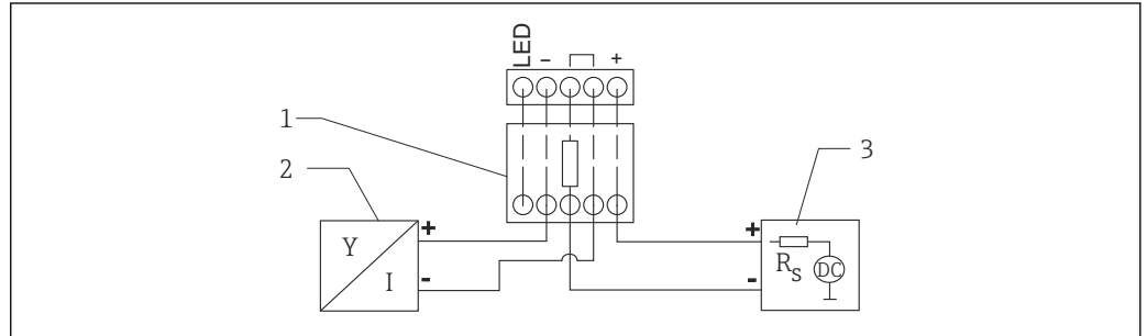
3 Block diagram; device connection, RIA15 without light, HART communication resistor
