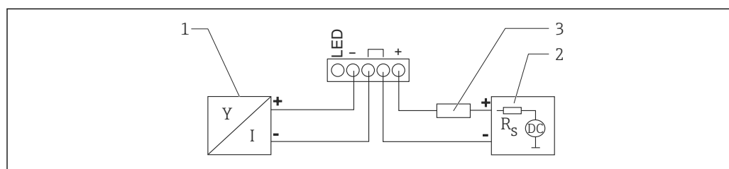
1 Block diagram; connection of the device with HART communication and RIA15 without backlighting
