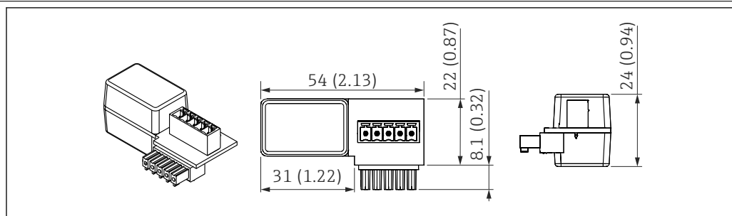
6 Dimensions of HART communication resistor. Unit of measurement mm (in)
