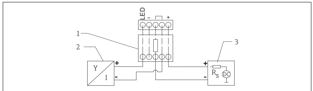
4 Block diagram; device connection, RIA15 with light, HART communication resistor module
