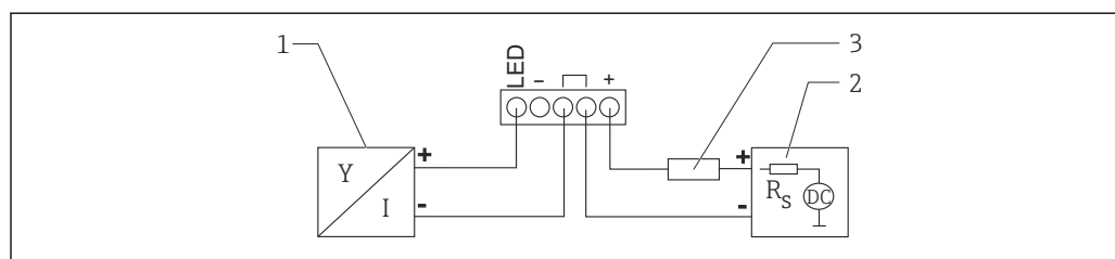
2 Block diagram; connection of the device with HART communication and RIA15 with backlighting
