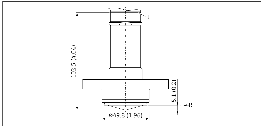
22 Dimensions; process connection NEUMO BioControl D50 PN16, 80 GHz; PEEK
