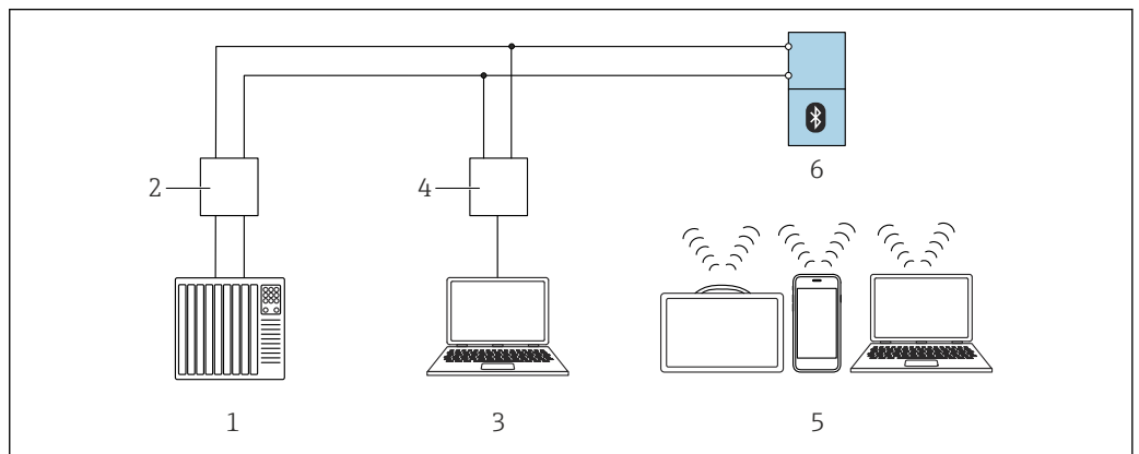
35 Options for remote operation via IO-Link
