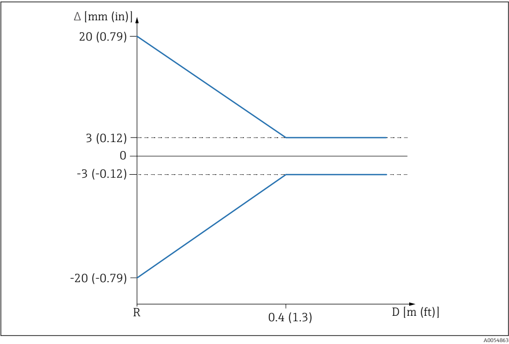
5 Maximum measurement error in near-range applications
