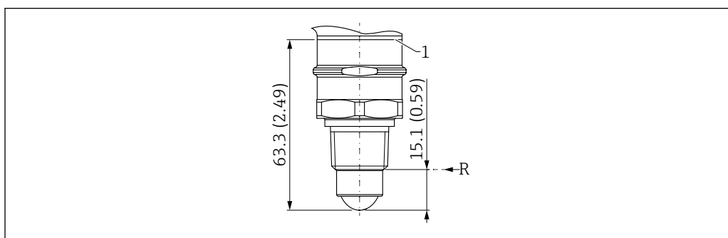
11 Dimensions; process connection MNPT ½, 180 GHz; PTFE
