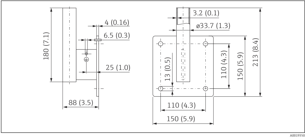
50 Dimensions of the wall bracket. Unit of measurement mm (in)
