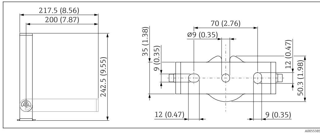
39 Dimensions of mounting bracket. Unit of measurement mm (in)
