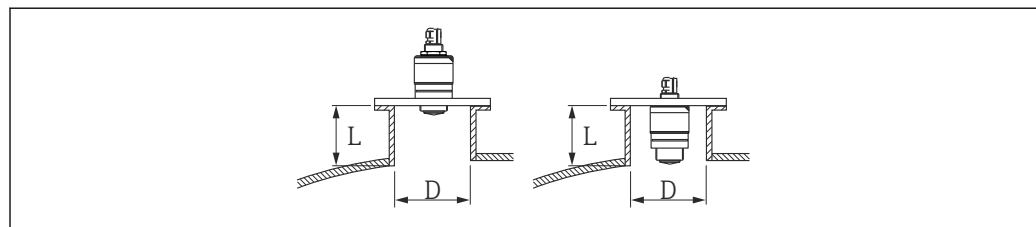
7 Nozzle mounting
