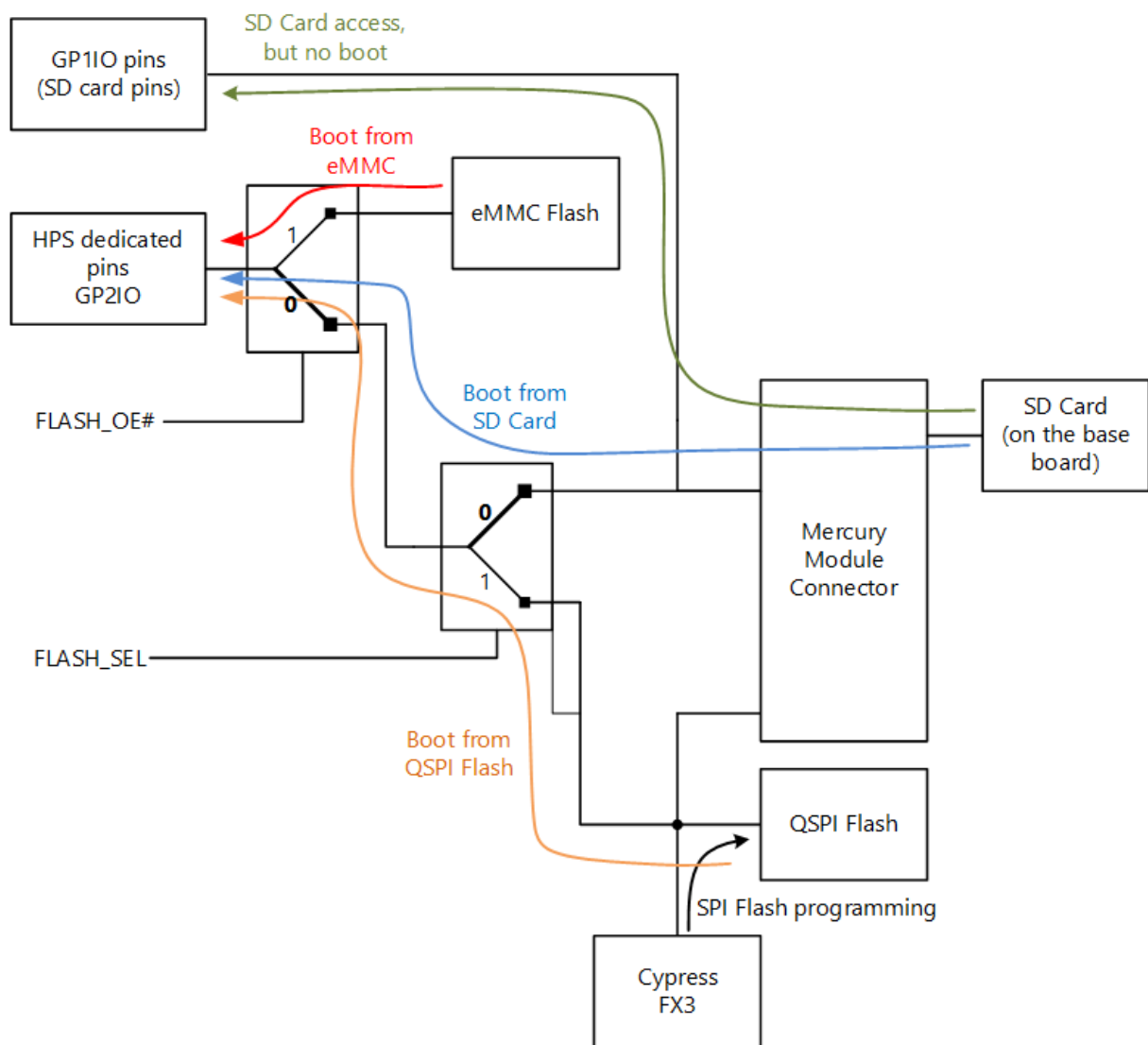
Figure 12: Boot Modes
