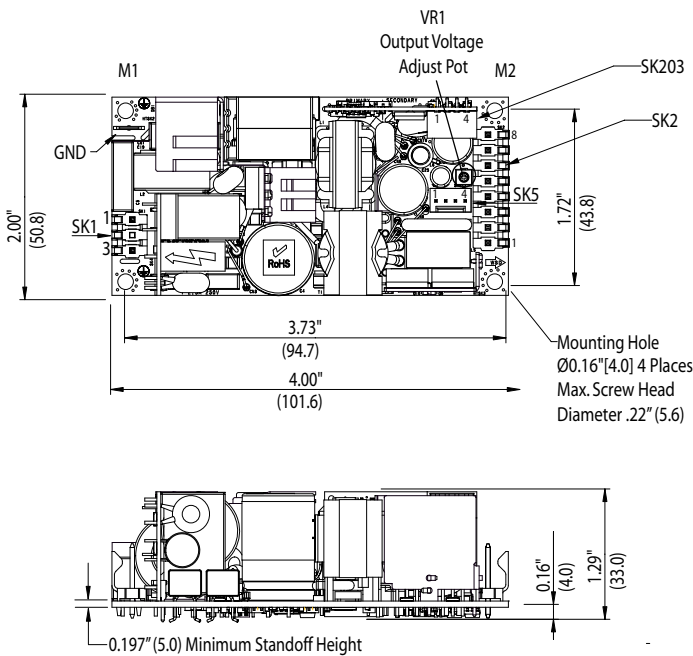
GL COMPACT SERIES CASE 1 AND 2 DIMENSIONS
