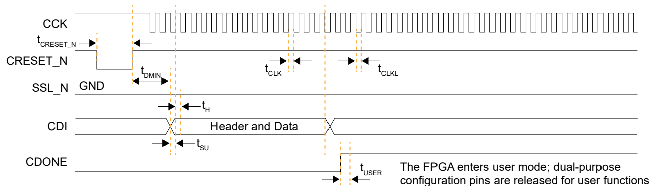
Figure 42: SPI Passive Mode (x1) Timing Sequence
