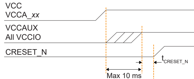
Figure 39: Power-Up Sequence
