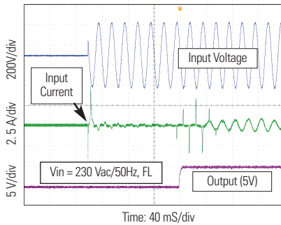
13. Turn-on Input Voltage & Input Current vs. Output Voltage
