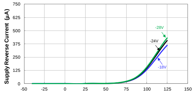
Temperature ( ^\circ\text{C} ) Supply Reverse Current vs Temperature
