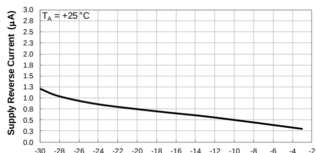
Supply Voltage (V) Supply Reverse Current vs Supply Voltage
