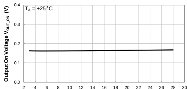
Supply Voltage (V) Output On Voltage vs Supply Voltage
