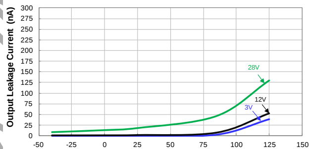
Temperature ( ^\circ\text{C} ) Output Leakage Current vs Temperature
