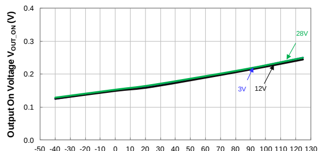
Temperature ( ^\circ\text{C} ) Output On Voltage vs Temperature
