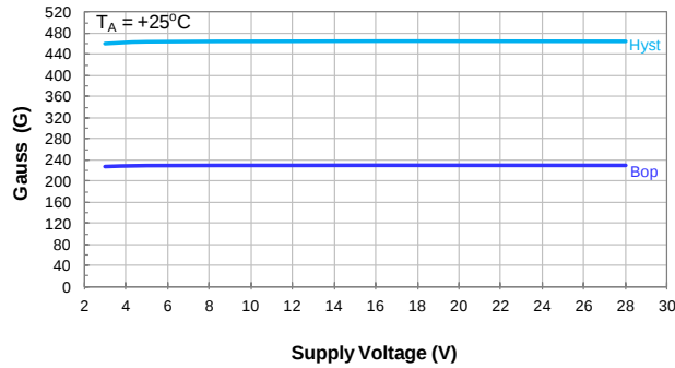
Switch Operate Point Bop vs Supply Voltage
