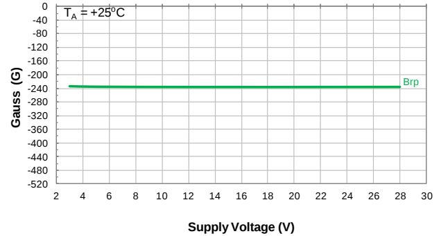
Switch Release Point Brp vs Supply Voltage
