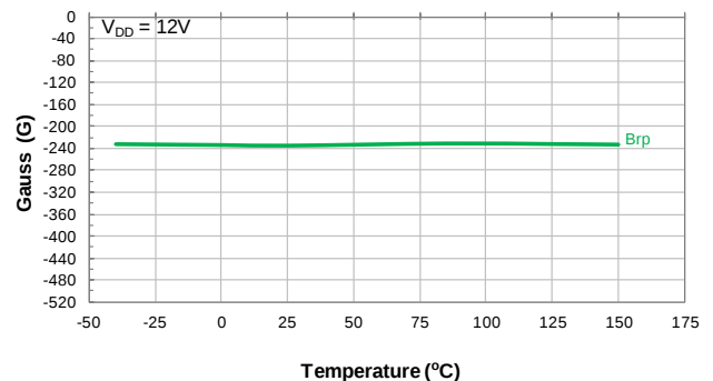
Switch Release Points Brp vs Temperature
