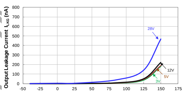
Temperature ( ^\circ\text{C} ) Output Leakage Current vs Temperature
