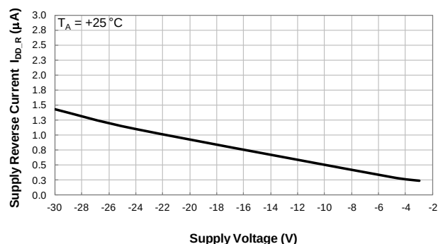
Supply Reverse Current vs Supply Voltage
