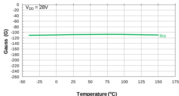
Switch Release Point Brp vs Temperature
