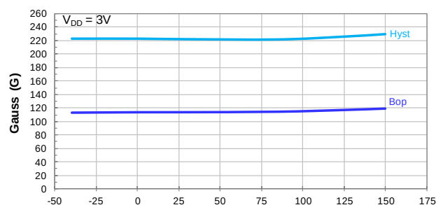
Temperature ( ^\circ\text{C} ) Switch Release Point Bop vs Temperature
