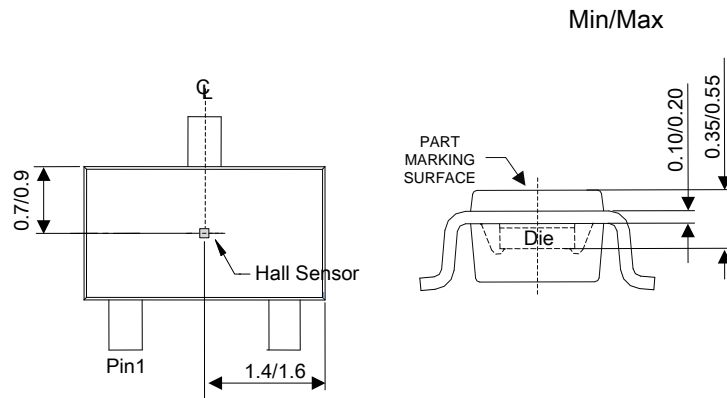
Sensor Location
