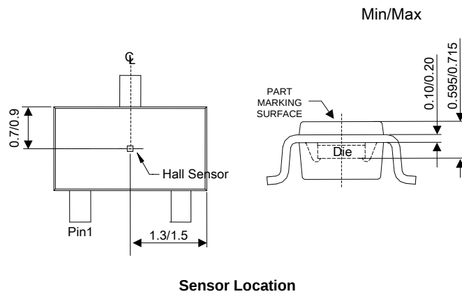
Sensor Location
