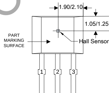
Sensor Location
