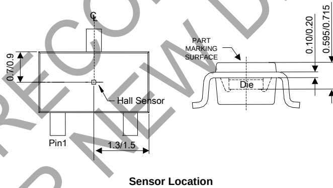
Sensor Location
