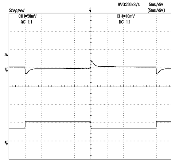
Figure 6: Output voltage response to step-change in load current (50%-75%-50% of I_o , max; di/dt = 0.1A/\mu s ). Load cap: 10\mu F , 100m\Omega ESR tantalum capacitor and 1\mu F ceramic capacitor. Top Trace: V_{out} (50mV/div), Bottom Trace: I_{out} (2A/div).
