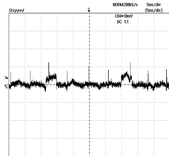
Figure 8: Input Reflected Ripple Current, i_s , at full rated output current and nominal input voltage with 12\mu H source impedance and 68\mu F electrolytic capacitor (2 mA/div).
