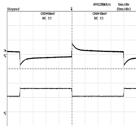
Figure 6: Output voltage response to step-change in load current (50%-75%-50% of I_o , max; di/dt = 0.1A/\mu s ). Load cap: 10\mu F , 100\text{ m}\Omega ESR tantalum capacitor and 1\mu F ceramic capacitor. Top Trace: V_{out} (50mV/div), Bottom Trace: I_{out} (2A/div).
