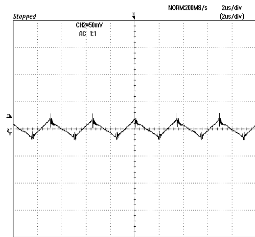
Figure 10: Output voltage ripple at nominal input voltage and rated load current (50 mV/div). Load capacitance: 1\mu F ceramic capacitor and 10\mu F tantalum capacitor. Bandwidth: 20 MHz.
