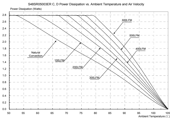
Figure 19: Power dissipation vs. ambient temperature and air velocity
