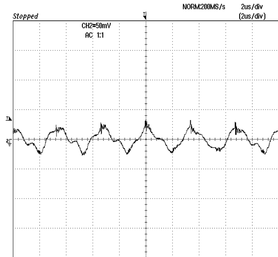
Figure 10: Output voltage ripple at nominal input voltage and rated load current (50 mV/div). Load capacitance: 1\mu\text{F} ceramic capacitor and 10\mu\text{F} tantalum capacitor. Bandwidth: 20 MHz.
