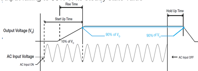
Figure 4 Time sequence
