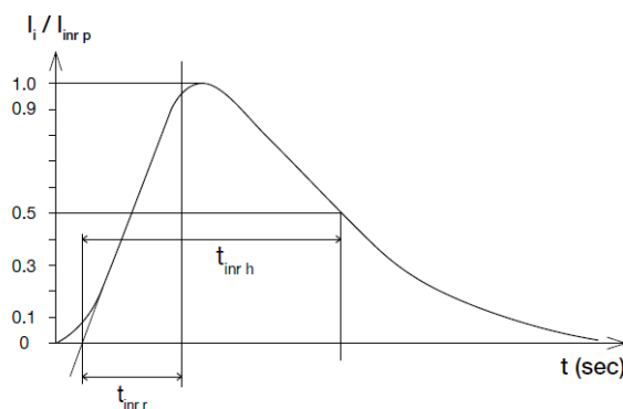
Figure 6 Inrush Current
