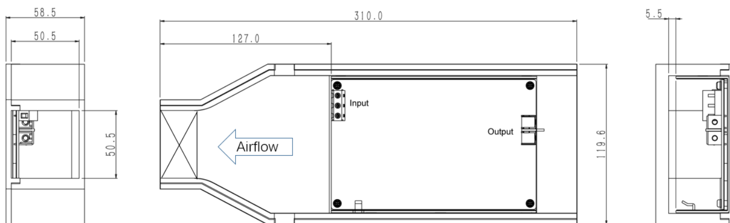
Thermal Fixture Setup. With Fan P/N: DELTA AFB0512HHD
