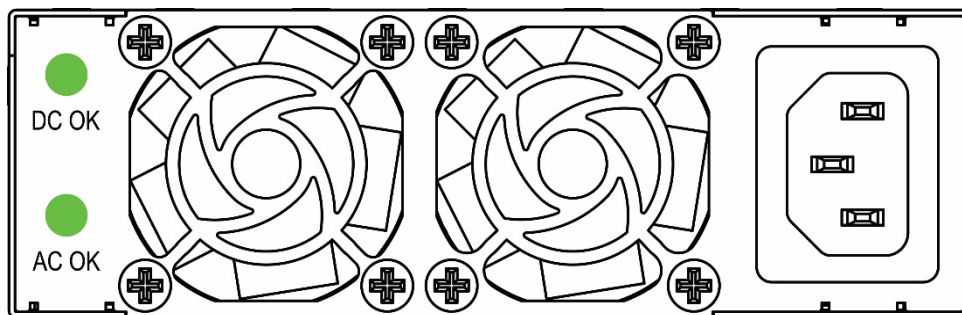
Figure 7. LED Indicator
