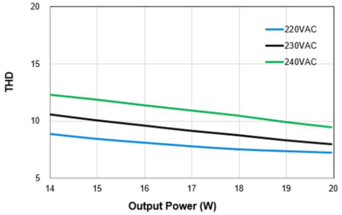
LNP-03A21WBCA – 350mA
