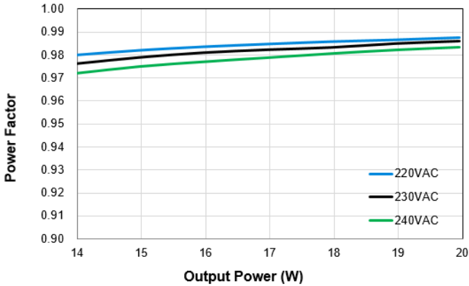
LNP-03A21WBCA – 350mA
