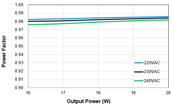
LNP-05A20WBCA – 500mA
