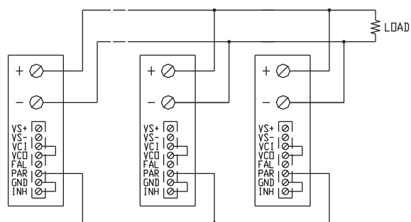
PARALLEL OPERATION WITHOUT REMOTE SENSING
