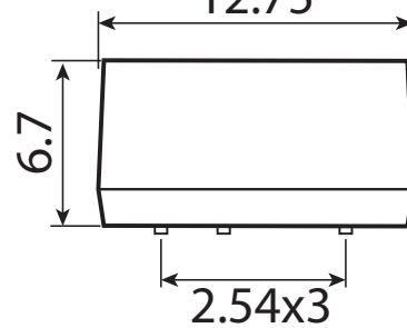
Side View 2.54x3
