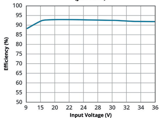
EFFICIENCY VS INPUT VOLTAGE PQC60-24-S24(-H) (full load)
