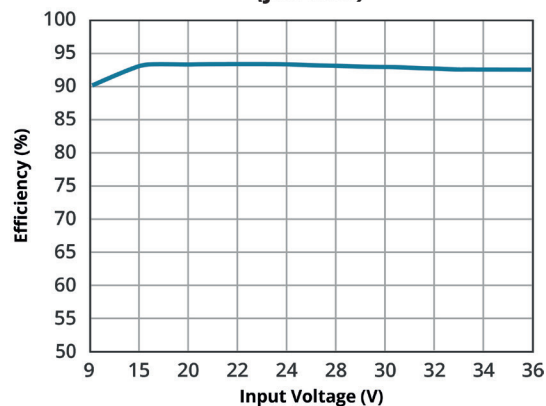
EFFICIENCY VS INPUT VOLTAGE PQC60-24-S15(-H) (full load)
