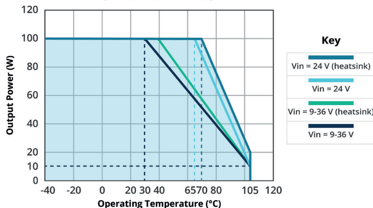
TEMPERATURE DERATING CURVE PQC60-24-S12 (natural convection)
