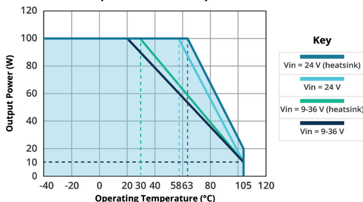
TEMPERATURE DERATING CURVE PQC60-24-S24 (natural convection)
