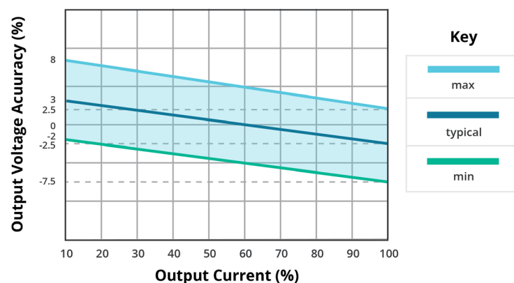
OUTPUT REGULATION CURVE
