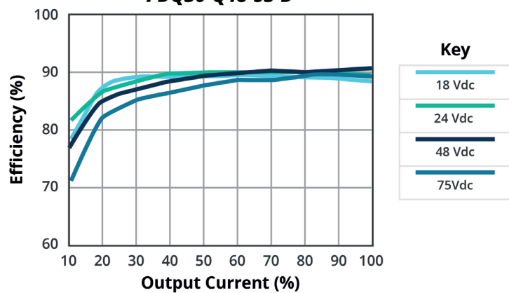
EFFICIENCY VS OUTPUT LOAD PDQ30-Q48-S5-D
