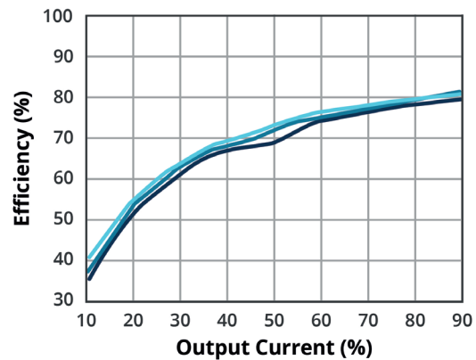
EFFICIENCY VS OUTPUT LOAD PCN1-S12-D15-S
