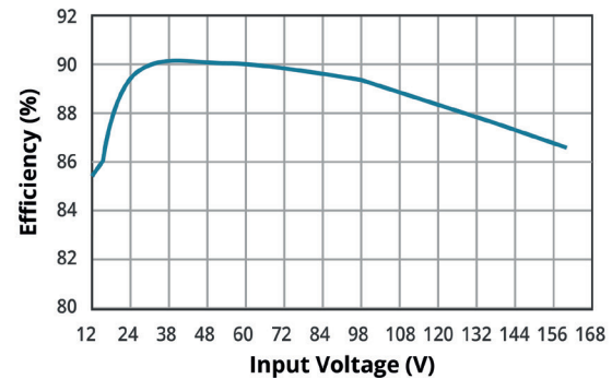
EFFICIENCY VS INPUT VOLTAGE (25°C, FULL LOAD) PVQ100W-072-S24-D
