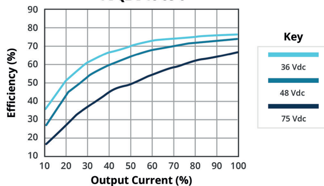
EFFICIENCY VS OUTPUT LOAD PDQ2-D48-S3-S
