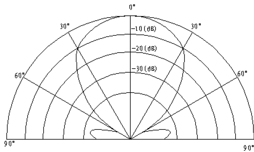
Directivity
