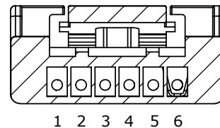
SECTION A-A SCALE 3 : 1 (Back of Connector Housing)
